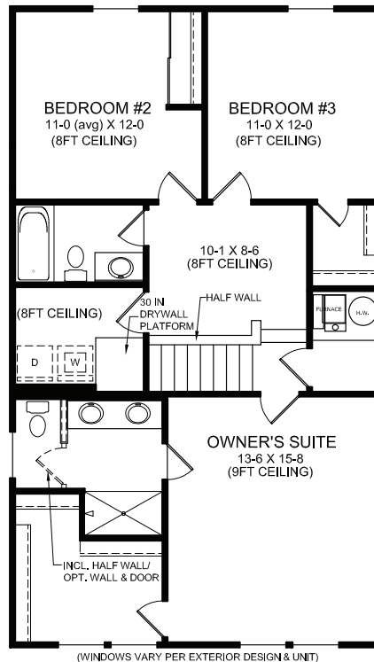
SECOND FLOOR DESIGN
