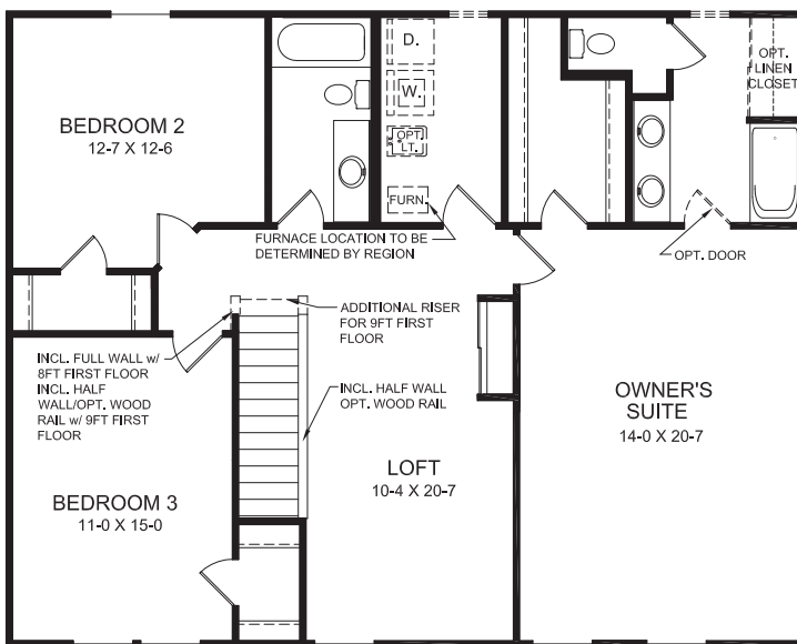
SECOND FLOOR DESIGN
