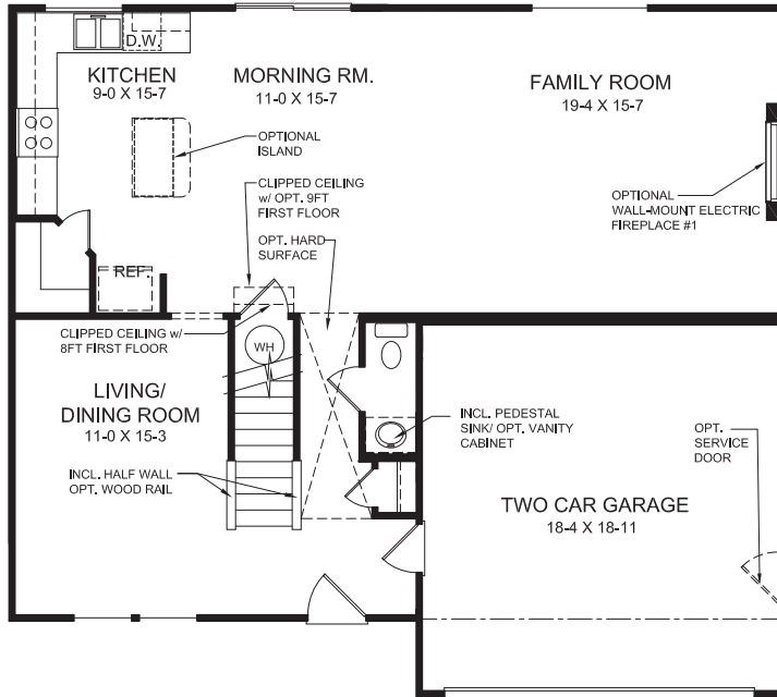
FIRST FLOOR DESIGN (STANDARD PLAN)
