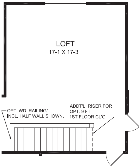
PARTIAL SECOND FLOOR DESIGN w/ OPT. BASEMENT
