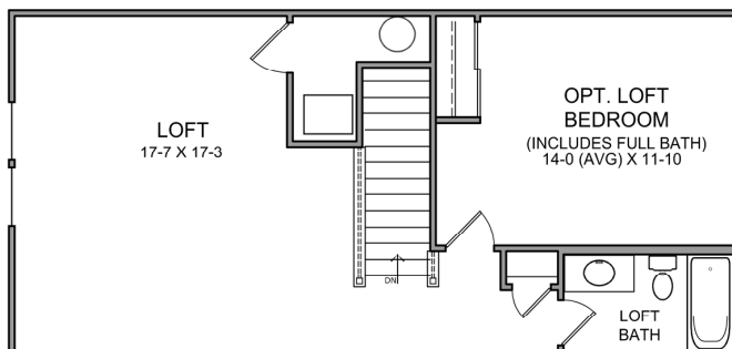
OPT. LOFT DESIGN SHOWN w/ OPT. BEDROOM AND FULL BATH
