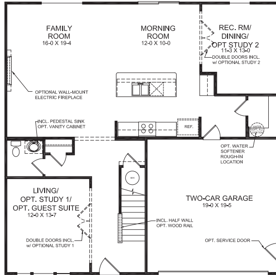
FIRST FLOOR DESIGN (STANDARD PLAN)
