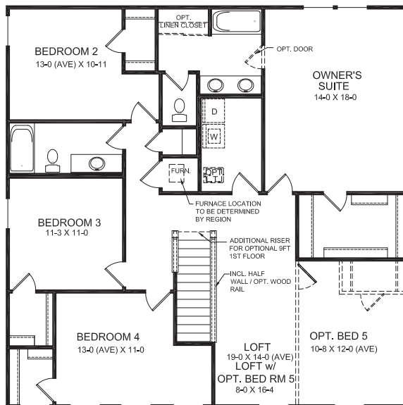
SECOND FLOOR DESIGN
