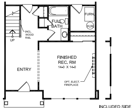
INCLUDED LOWER LEVEL DESIGN SHOWN w/ OPTIONAL FULL BATH
